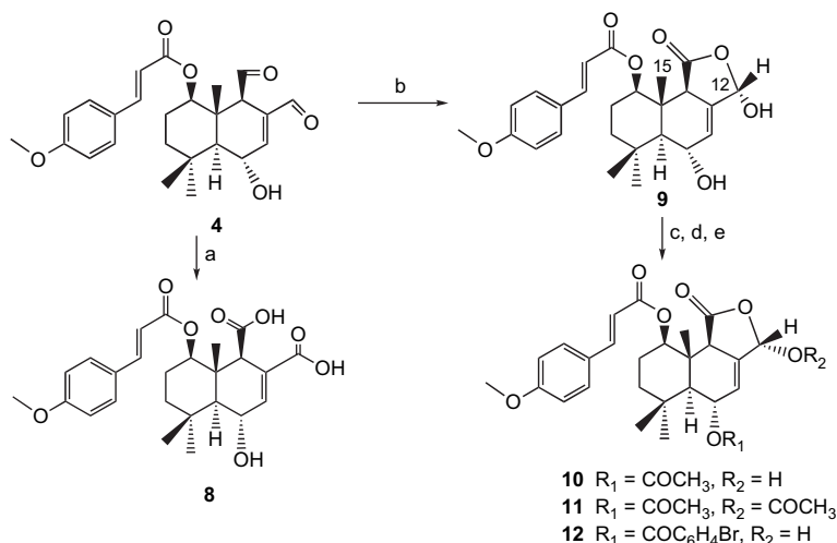
Scheme 2. Reagents and conditions: (a) \text{NaClO}_2 (5 equiv), \text{H}_2\text{O}_2 (4 equiv), acetonitrile, rt, 96%; (b) \text{NaClO}_2 (2 equiv), \text{NH}_2\text{SO}_3\text{H} (2 equiv), 1,4-dioxane/water (4:1), 0^\circ\text{C} , 94%; (c) \text{CH}_3\text{COCl} (1.1 equiv), pyridine (1.1 equiv), \text{CH}_2\text{Cl}_2 , rt, 25%; (d) \text{CH}_3\text{COCl} (3.3 equiv), pyridine (3.3 equiv), \text{CH}_2\text{Cl}_2 , rt, 31%; (e) DCC (1.1 equiv), DMAP (0.2 equiv), \text{BrC}_6\text{H}_4\text{CO}_2\text{H} (1.1 equiv), toluene, rt, 50%.
